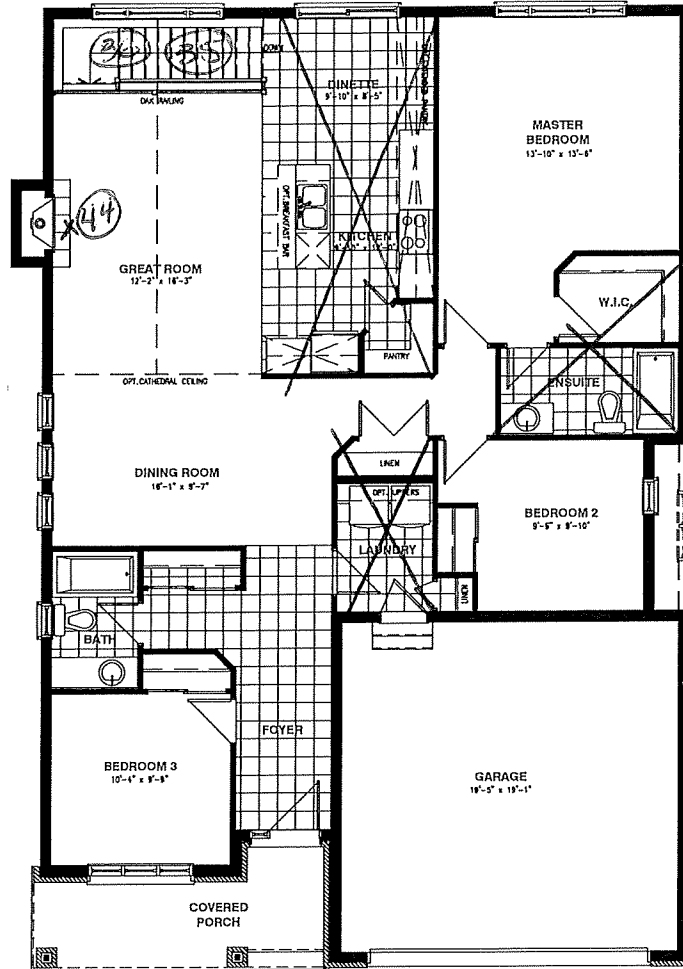
GROUND FLOOR - ELEVATION A & B
