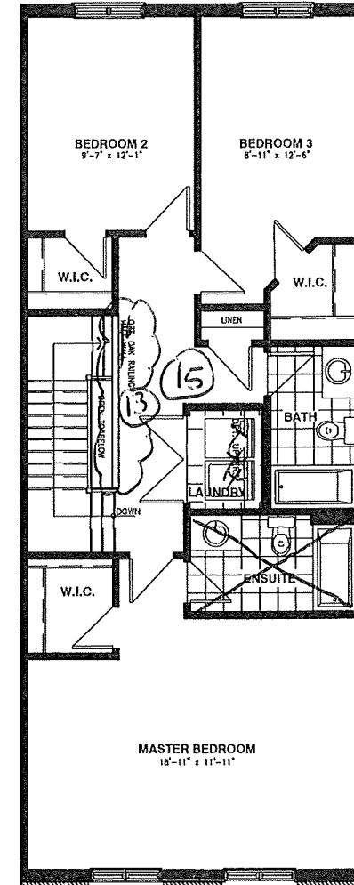
SECOND FLOOR
