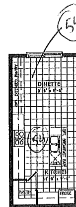
OPTIONAL KITCHEN #1
