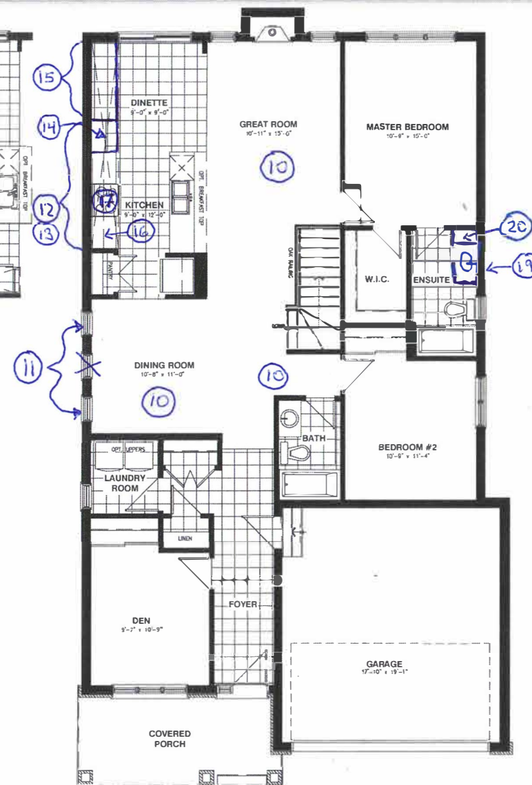
GROUND FLOOR - ELEVATION C
