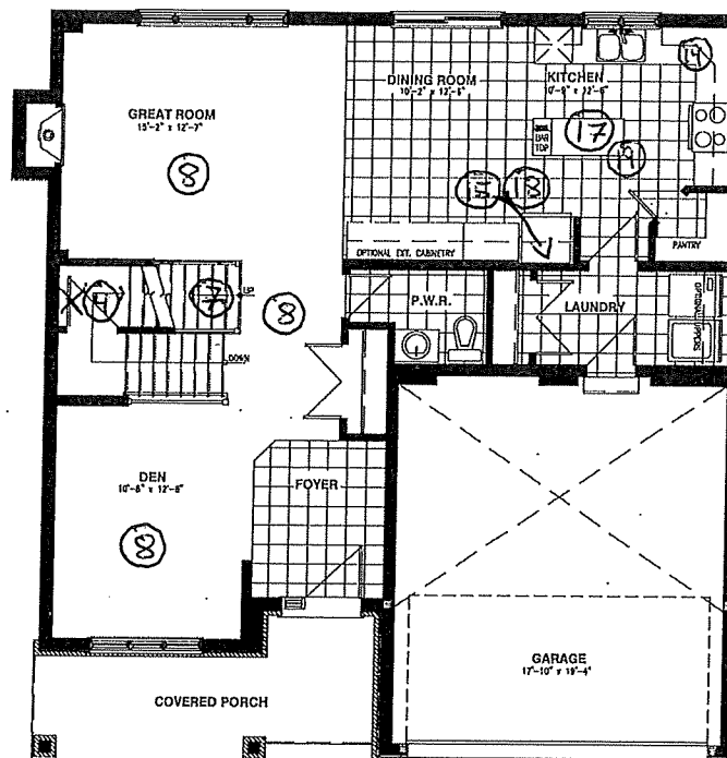
GROUND FLOOR - ELEVATION A & B
