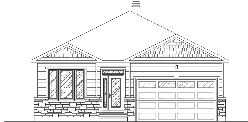
ELEVATION C
