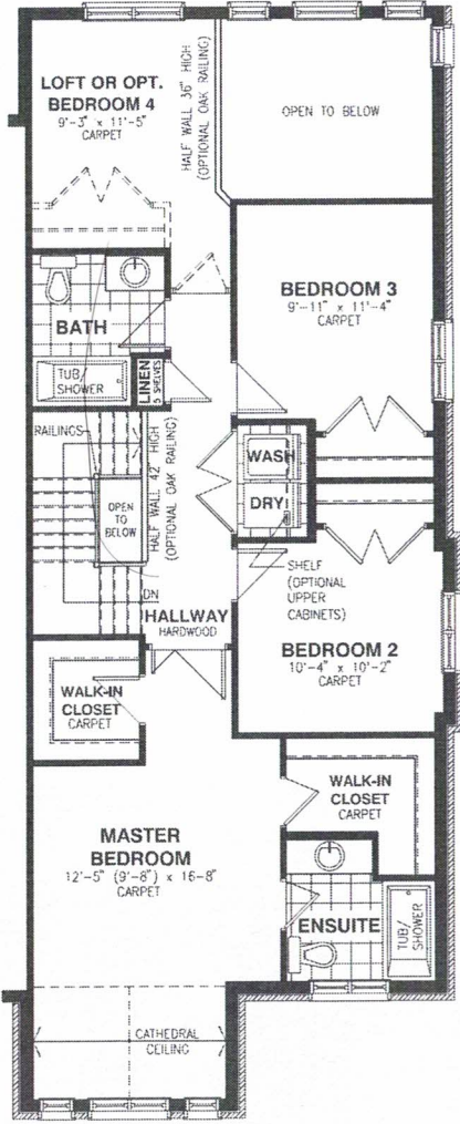
SECOND FLOOR
