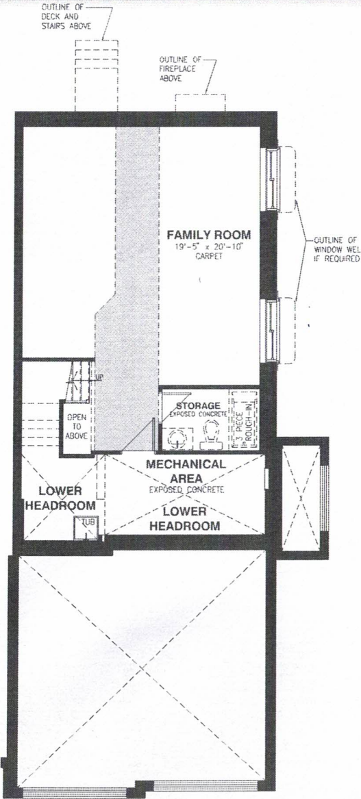
BASEMENT FLOOR
