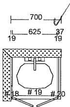
POWDER ROOM
