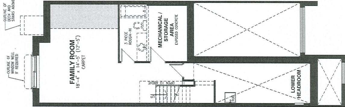
BASEMENT FLOOR
