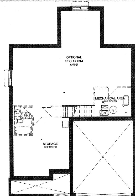
BASEMENT FLOOR - ELEVATION A & C
