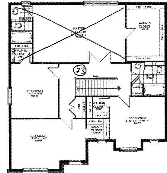
SECOND FLOOR-ELEVATION A
