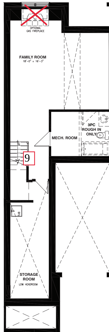
BASEMENT FLOOR
