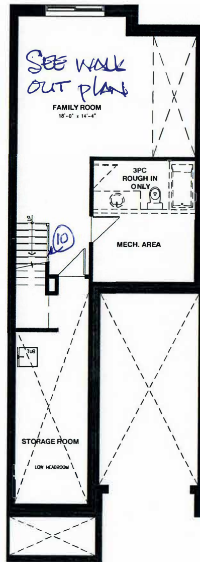
BASEMENT FLOOR
