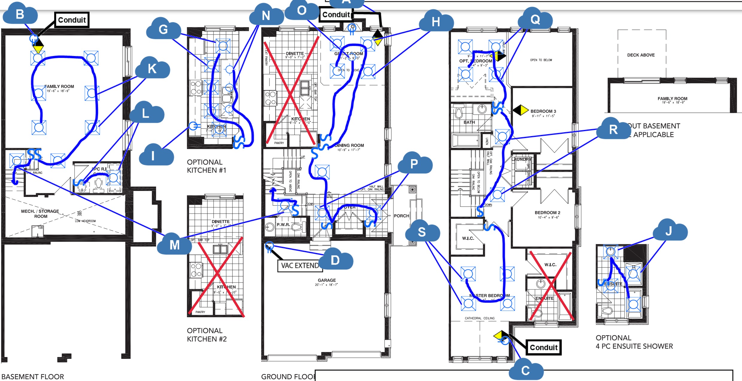
BASEMENT FLOOR
