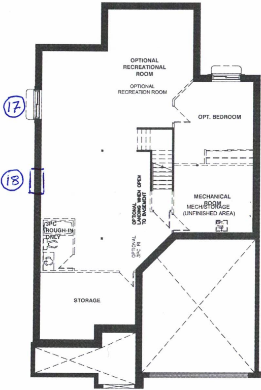
BASEMENT FLOOR - ELEVATION A & C
