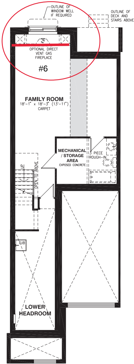
BASEMENT FLOOR
