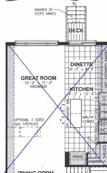
OPTIONAL KITCHEN #2
