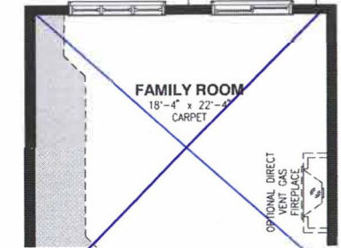
WALKOUT BASEMENT WHERE APPLICABLE
