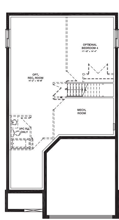
BASEMENT FLOOR
