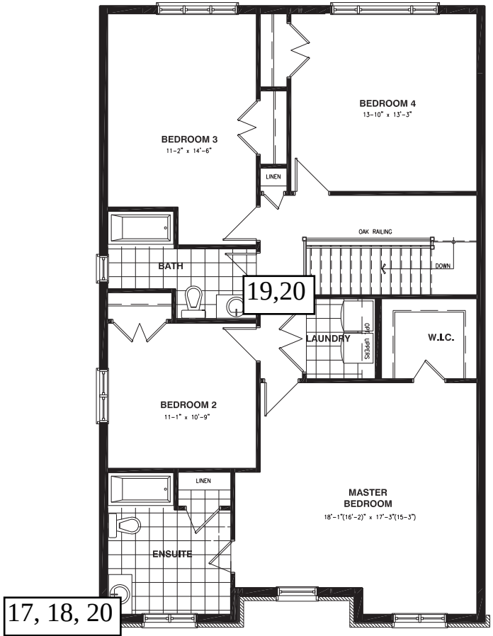
SECOND FLOOR - 4 BEDROOMS - ELEVATION A
