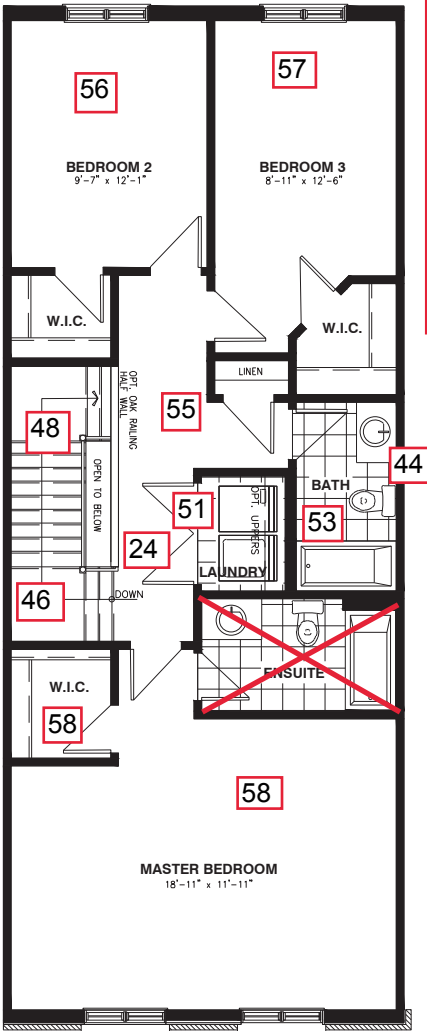
SECOND FLOOR
