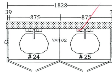
ENSUITE 2ND FLOOR
