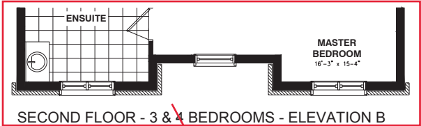
SECOND FLOOR - 3 & 4 BEDROOMS - ELEVATION B
