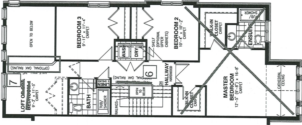
SECOND FLOOR
