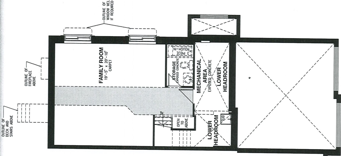
BASEMENT FLOOR
