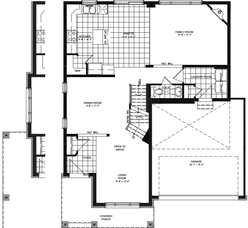
GROUND FLOOR - ELEVATION A
