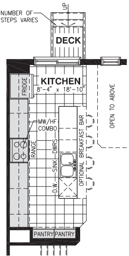
OPTIONAL KITCHEN #1
