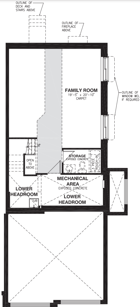
BASEMENT FLOOR
