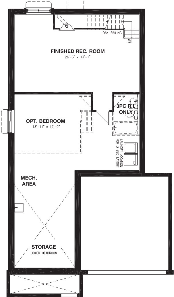
BASEMENT FLOOR
