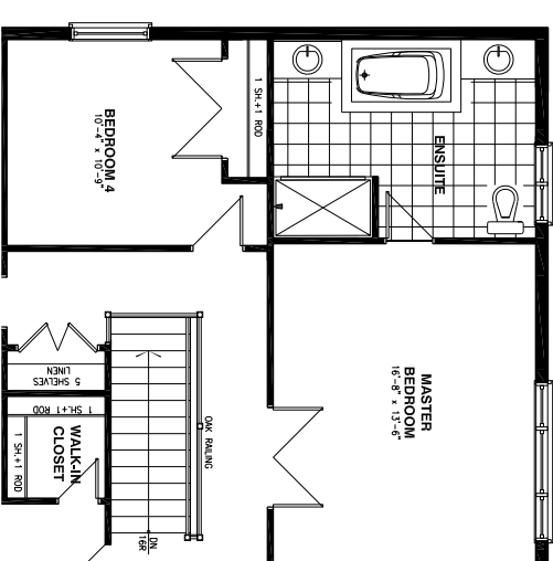
5PC Ensuite Upgrade
