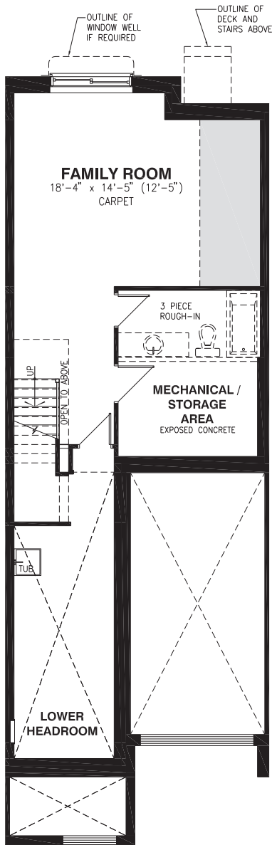
BASEMENT FLOOR
