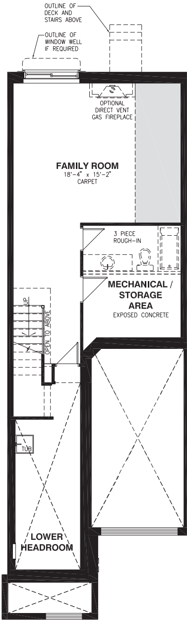
BASEMENT FLOOR
