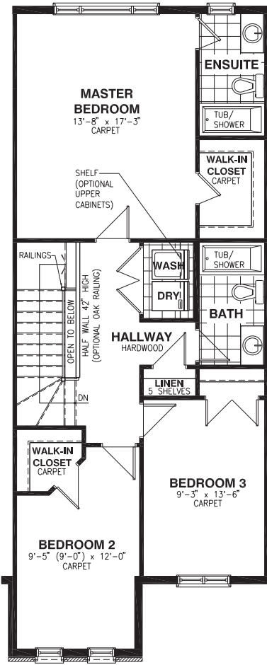
SECOND FLOOR
