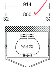
OPT. 4PC ENSUITE 2ND FLOOR
