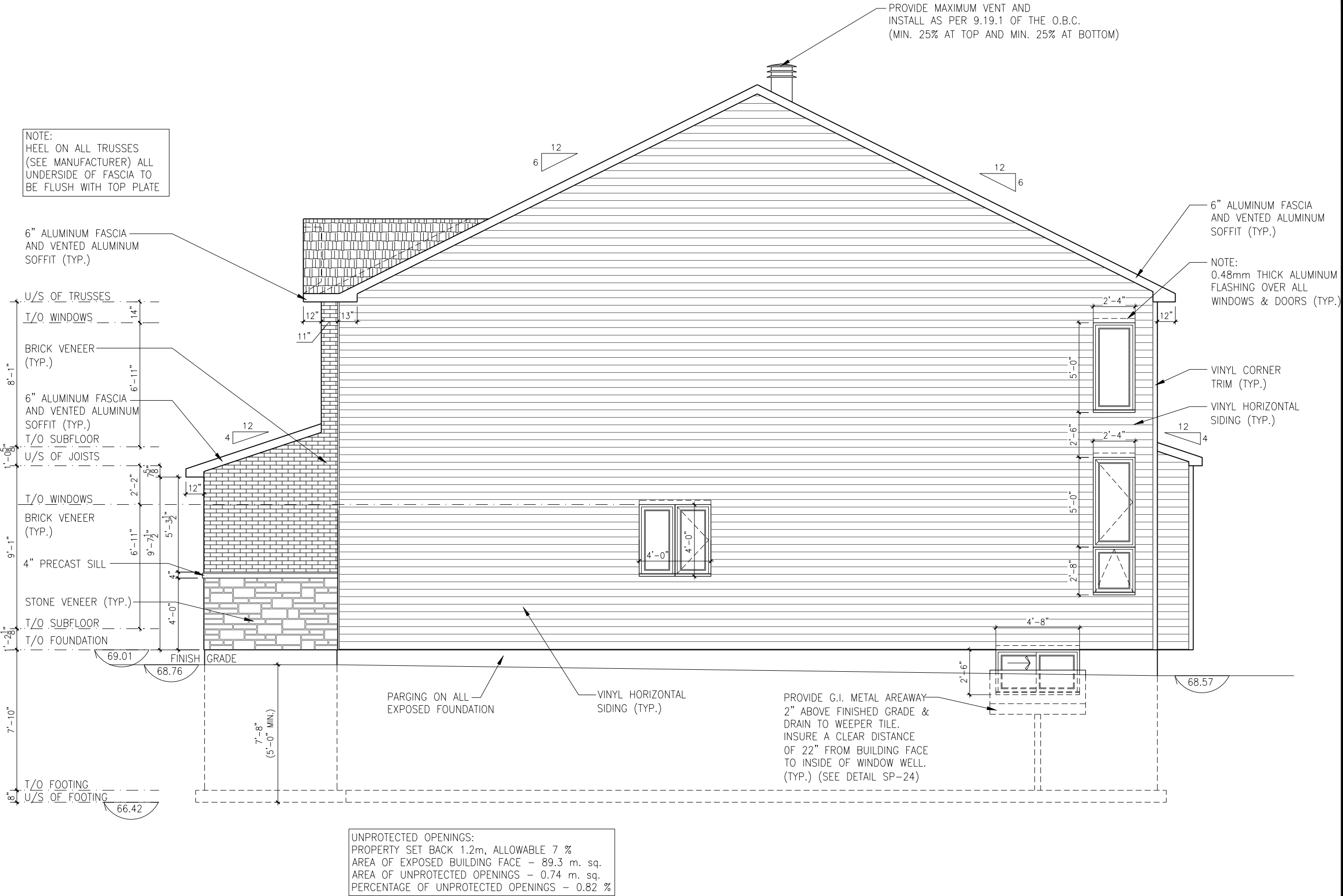
RIGHT ELEVATION - 3 BEDROOM - ELEVATION A SCALE: 3/16" = 1'-0"
