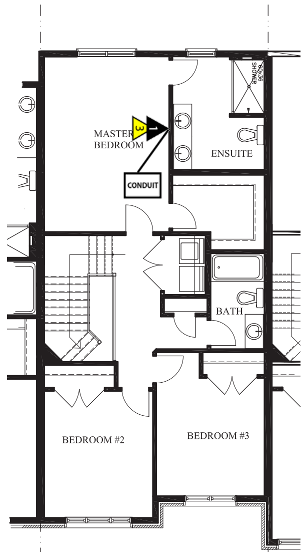
817.89sq.ft. SECOND FLOOR
