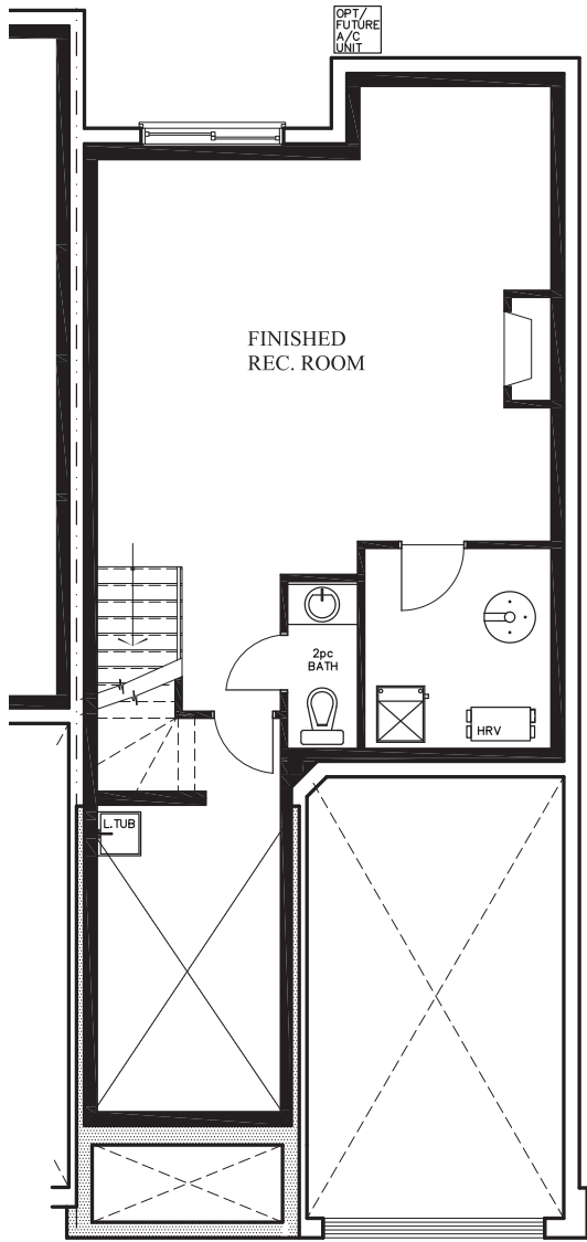
499.42 sq.ft. fin bsmt BASEMENT FLOOR
