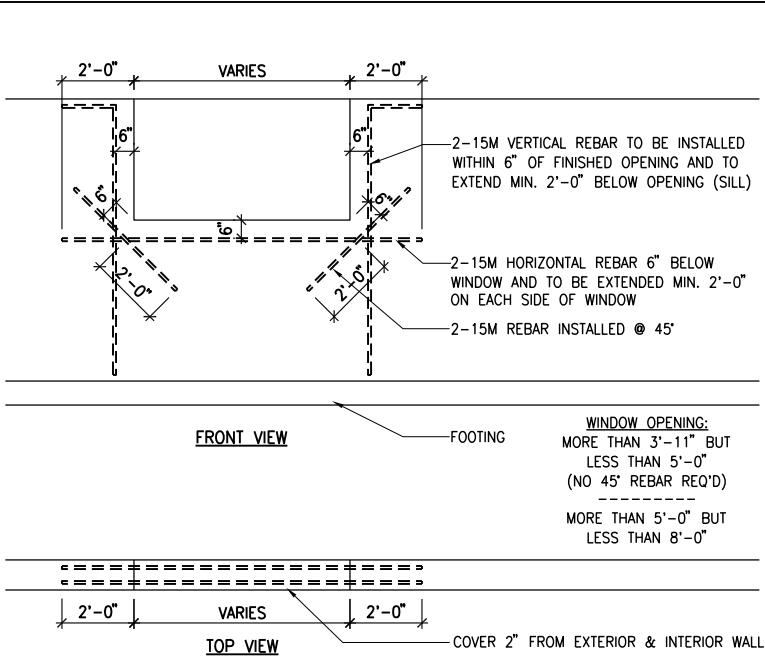
2 A.4f BASEMENT WINDOW REINFORCING SCALE: 3/16" = 1'-0"
