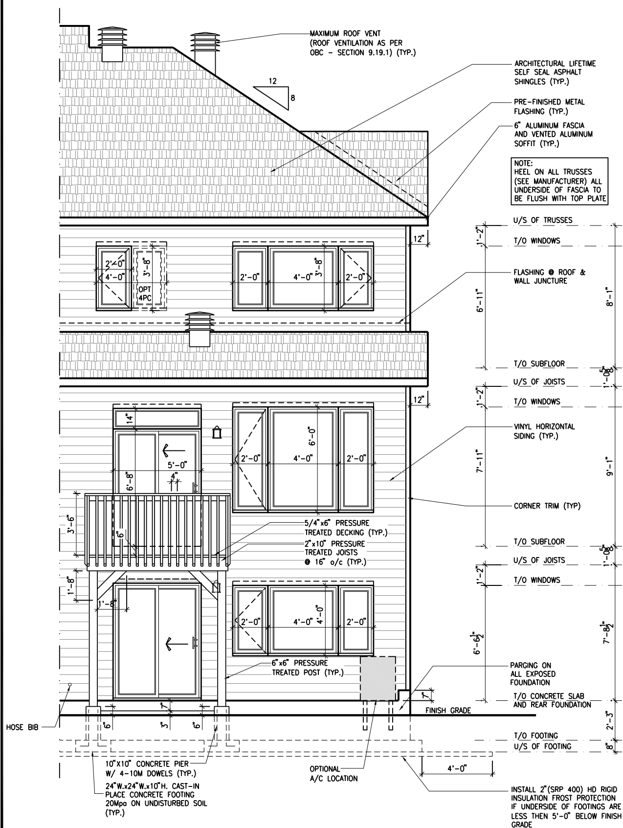
2 REAR ELEVATION - PORCH END UNIT - WALKOUT
