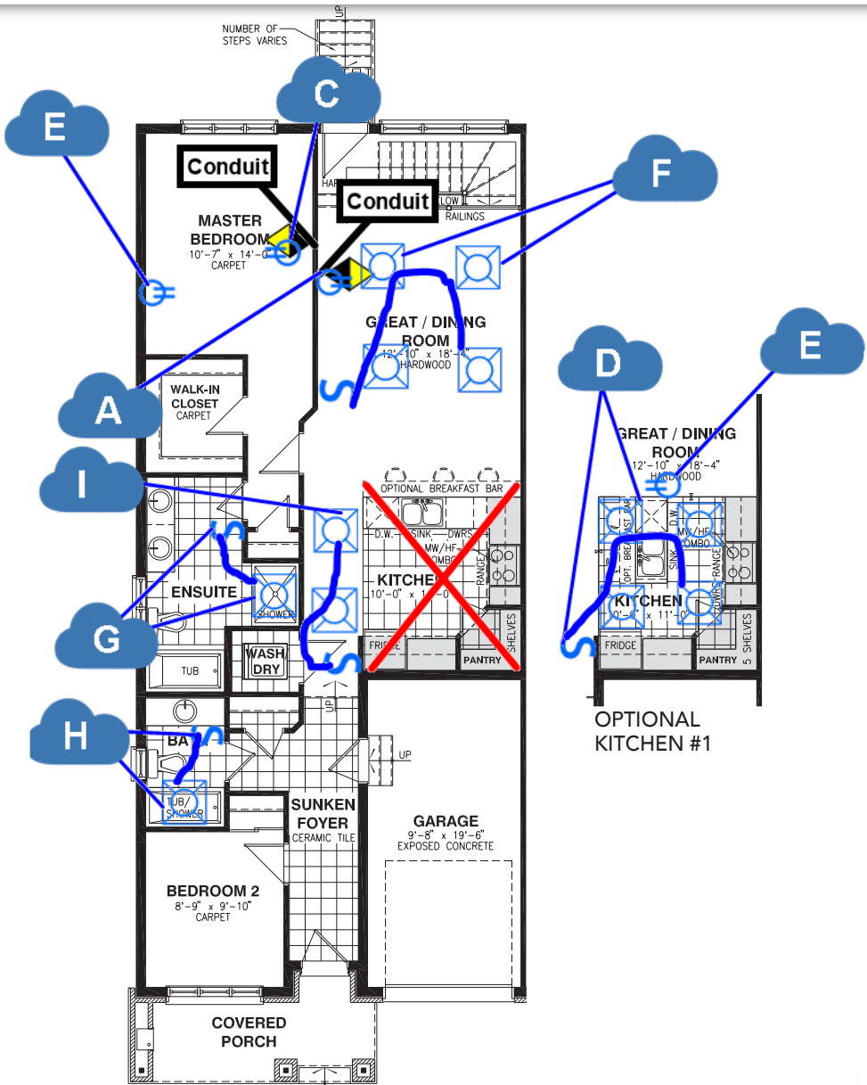
GROUND FLOOR OPTIONAL 2 BEDROOM
