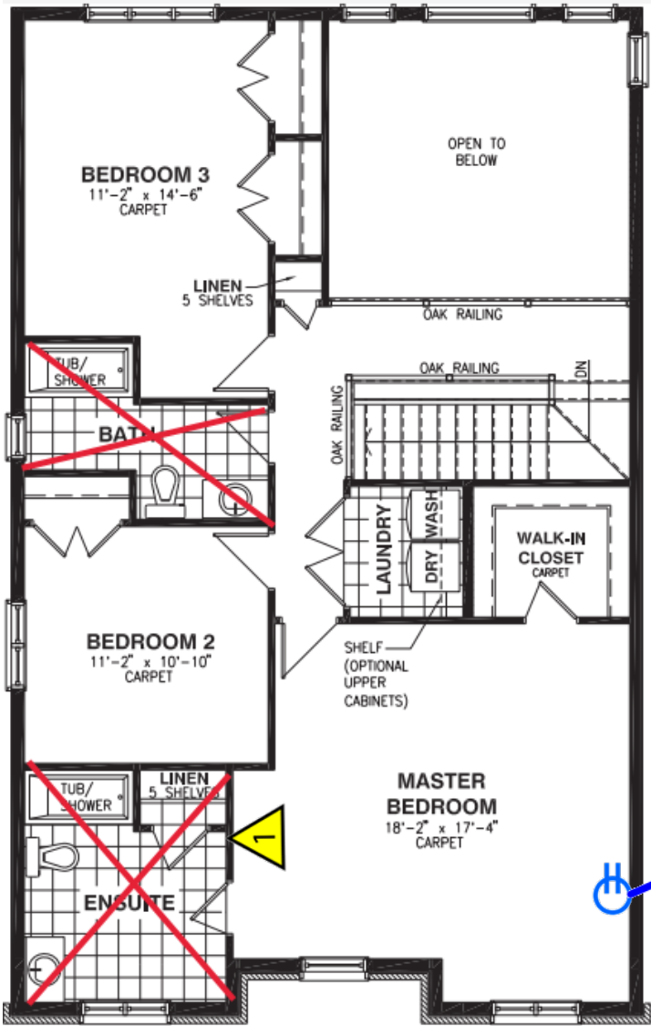
SECOND FLOOR - 3 BEDROOMS - ELEVATION A
