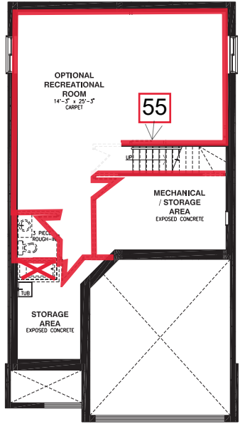
BASEMENT FLOOR
