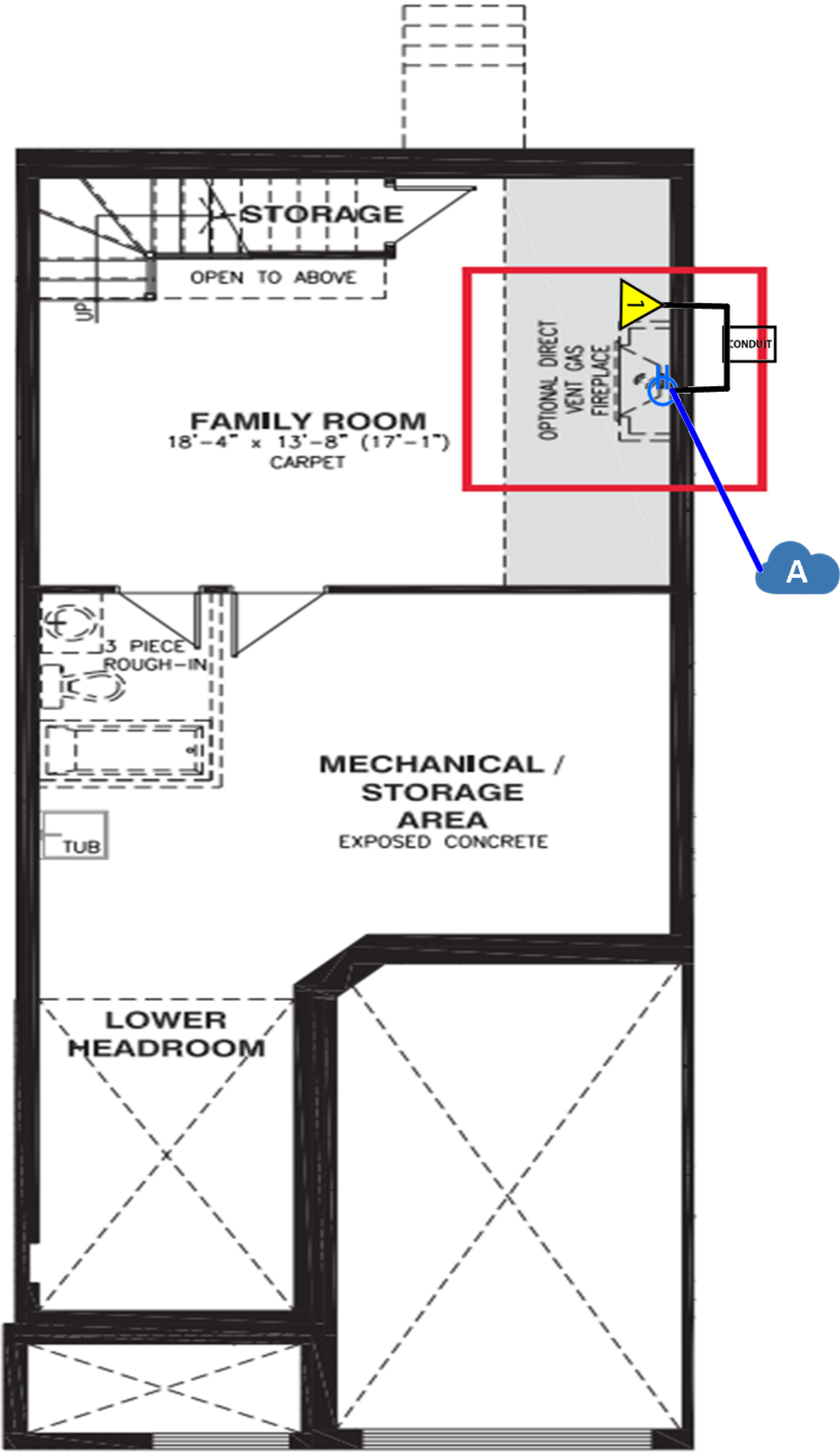
BASEMENT FLOOR
