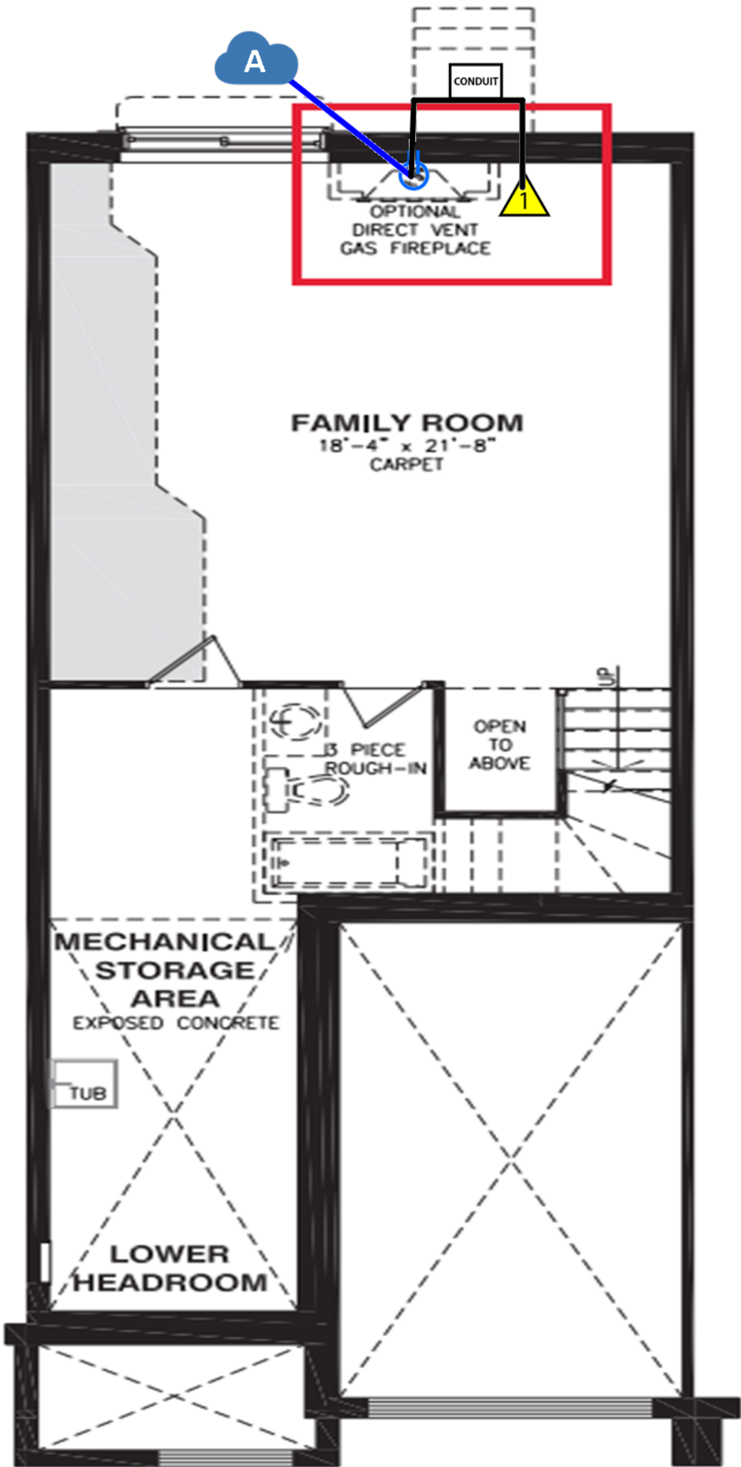
BASEMENT FLOOR
