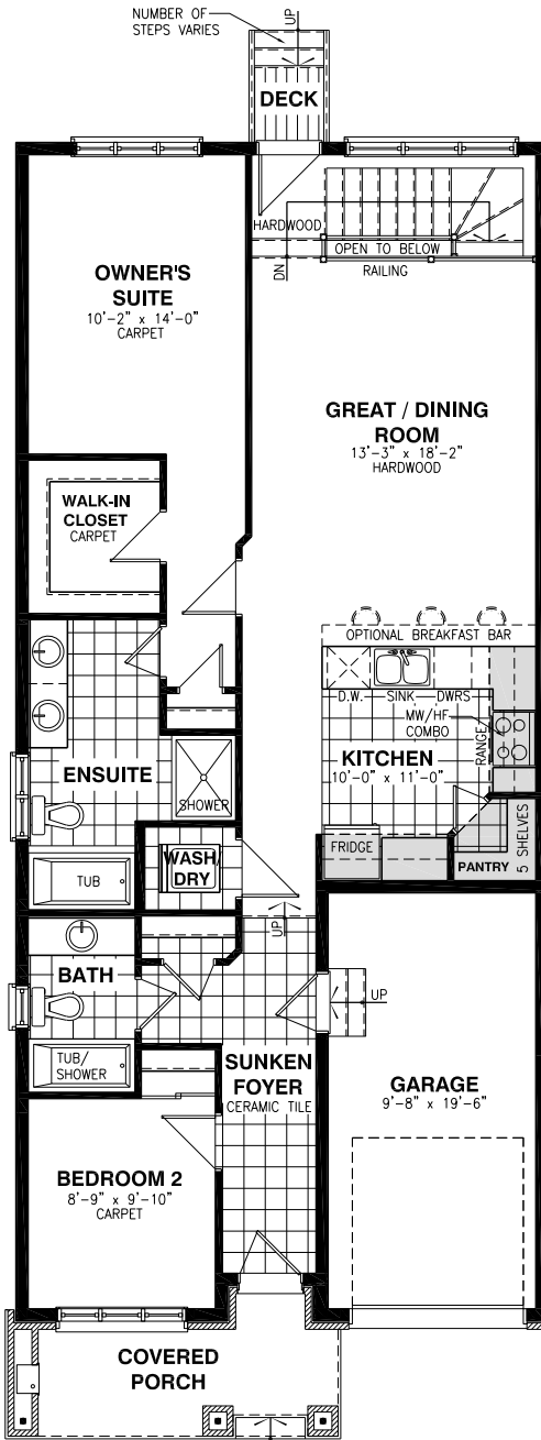
GROUND FLOOR PLAN OPTIONAL 2 BEDROOM
