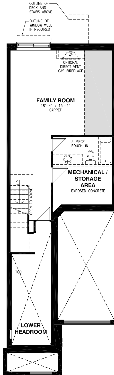
BASEMENT FLOOR PLAN
