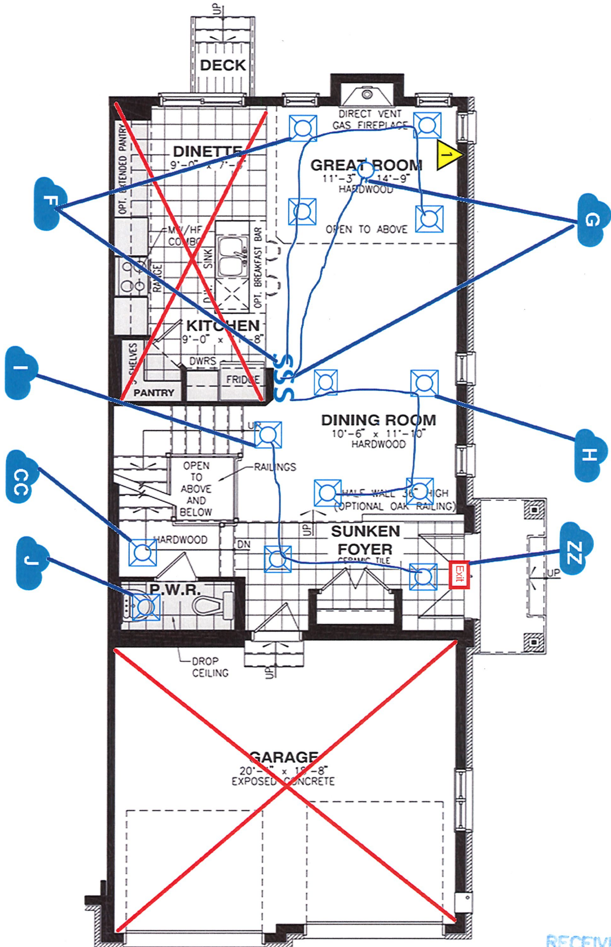
GROUND FLOOR
