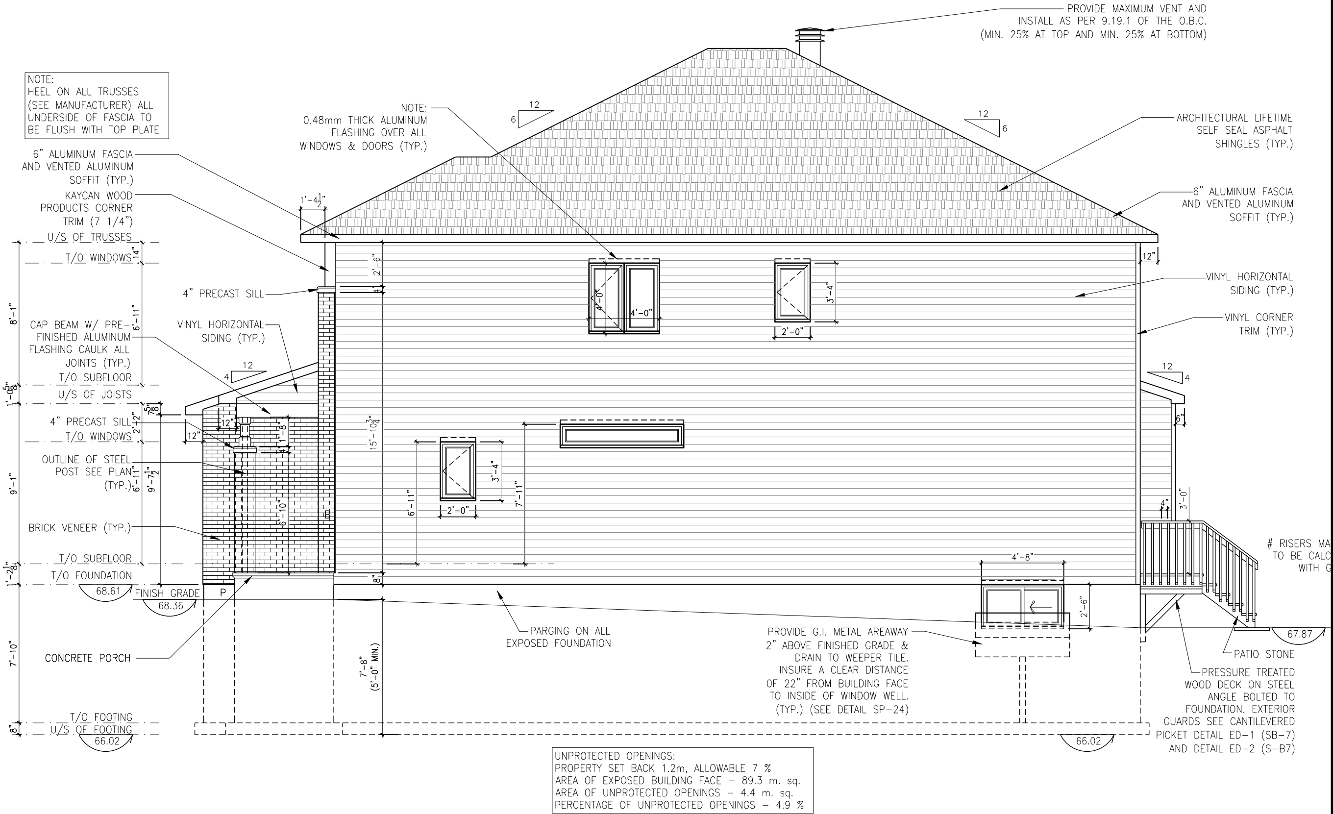
LEFT ELEVATION - 3 AND 4 BEDROOM - ELEVATION B
