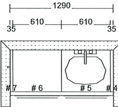
ENSUITE (4PC) 2ND FLOOR Floating Vanity w/ MDF build up
