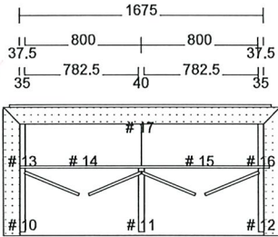
OPT LAUNDRY 2ND FLOOR 914mm UPFERS INSTALL CAB 1479mm FROM FINISHED FLOOR
