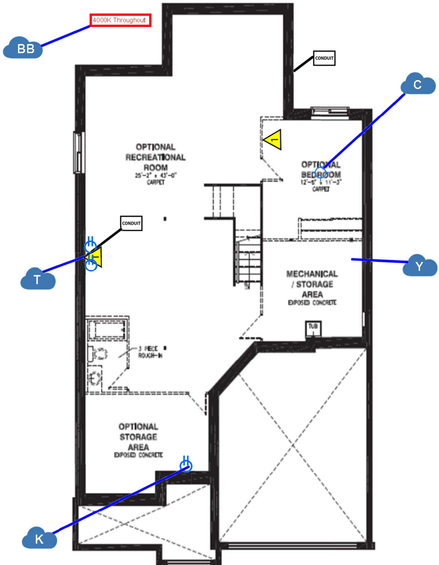
BASEMENT FLOOR - ELEVATION A
