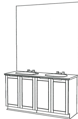
OPT 5PC ENSUITE 2ND FLOOR LOCATE SINKS ACCORDING TO MOUNTED LIGHT FIXTURES
