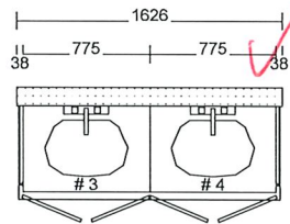
OPT 5PC ENSUITE 2ND FLOOR LOCATE SINKS ACCORDING TO MOUNTED LIGHT FIXTURES
