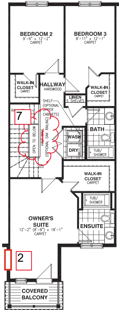
SECOND FLOOR
