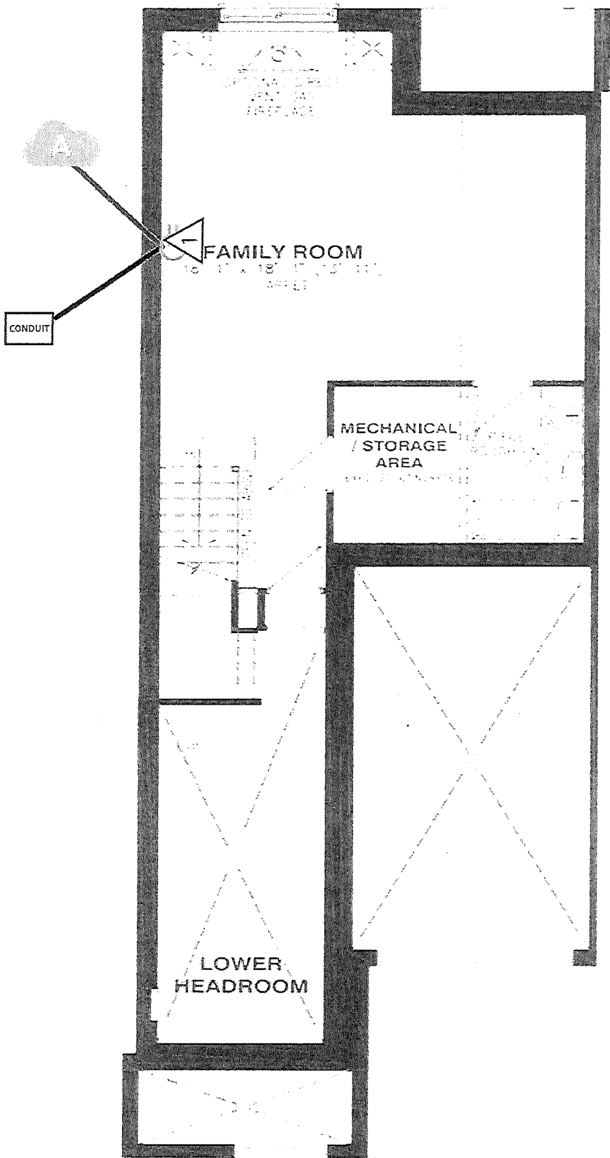
BASEMENT FLOOR
