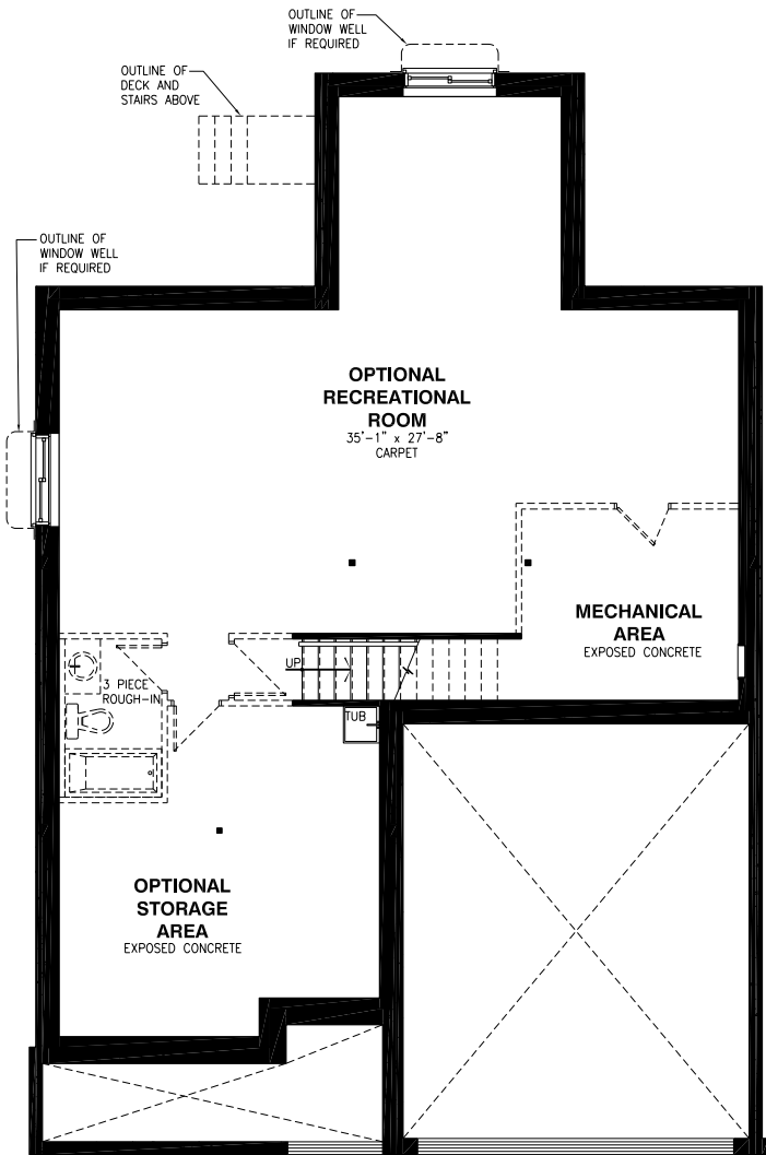
Basement Floor - Elevation A and B
