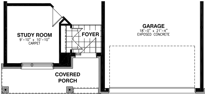
Ground Floor - Elevation B
