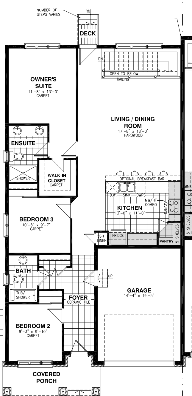
GROUND FLOOR PLAN STANDARD 3 BEDROOM
