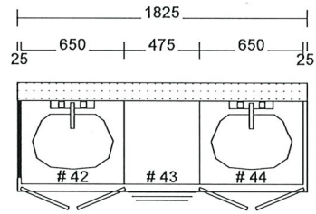
5PC ENSUITE ELEV 'B' 2ND FLOOR
