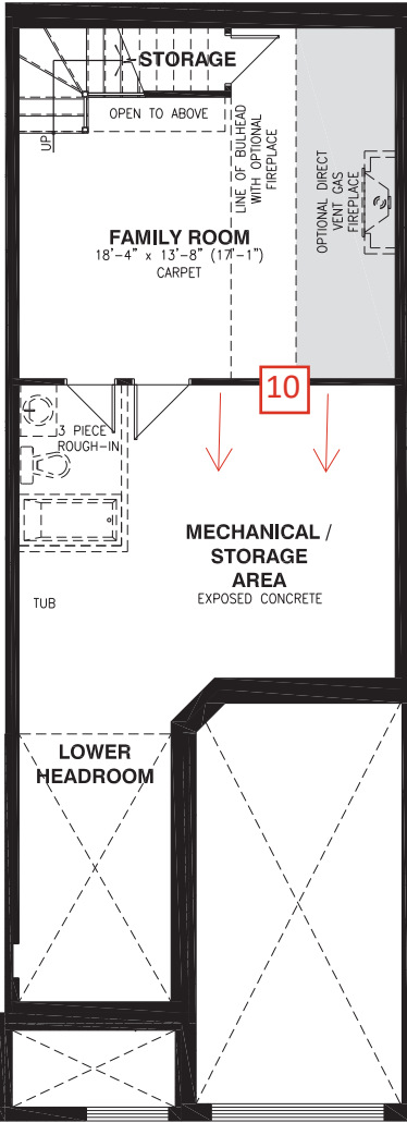
BASEMENT FLOOR
